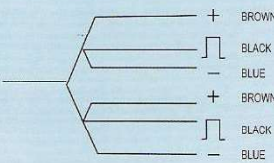
TYPES EQ, E2Q & E3Q (QUADRATURE)
