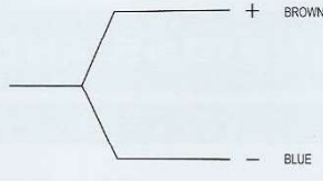
TYPE N (NAMUR) 5 - 25Vdc
